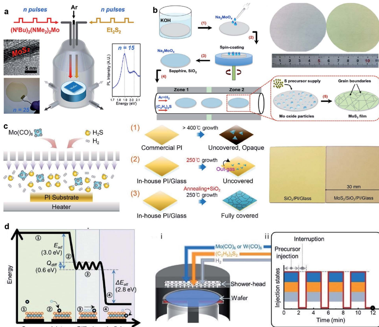
Fig. 5 (a) Schematic of pulsed MOCVD growth for 2H-MoS 2 in a single-wafer reactor geometry via pulsed injections of (\text{NBu})_2(\text{NMe}_2)_2\text{Mo} and \text{Et}_2\text{S}_2 . 53 Reproduced with permission from ref. 53, copyright 2017 American Chemical Society. (b) Schematic illustration of wafer-scale MoS 2 film growth process and photos of the 2-inch wafers of clean sapphire substrate (left) and the as-grown MoS 2 /sapphire (right). 56 Inset: The proposed mechanism for MoS 2 growth on the substrates. Reproduced with permission from ref. 56, copyright 2019 Springer Nature. (c) Schematic of the direct growth process of MoS 2 on the PI substrate: (1) PI is changed to opaque and sparse MoS 2 islands are grown; (2) the growth of MoS 2 at 250 °C. (3) The heat-annealing and capping procedures prevent the outgassing phenomenon and further absorption in the ambient environment, forming fully-covered MoS 2 . 21 Reproduced with permission from ref. 21, copyright 2019 American Chemical Society. (d) Calculated reaction energy diagram of Mo adsorbed on the basal plane of MoS 2 and the schematic illustration of (i) the reactor geometry and (ii) injection sequence of the precursors for growing wafer-scale monolayer TMD by pulsed MOCVD. 57 Reproduced with permission from ref. 57, copyright 2020 John Wiley and Sons.
