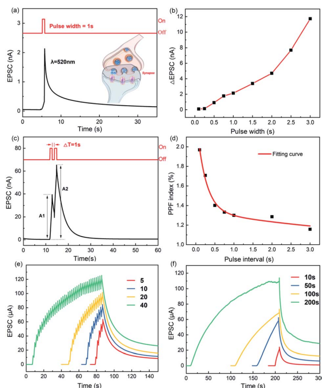
Fig. 4 (a) The EPSC triggered by optical pulse (520 nm, 1 s) at a drain voltage of 10 mV and a gate voltage of −20 V. Inset: Schematic diagram of the signal propagation of neurons. (b) The variation of the EPSC as a function of the optical pulse width. (c) EPSC induced by two 1 s light spikes (520 nm, \Delta T = 1 s), and (d) PPF index at different pulse intervals. (e) The change from short-term plasticity to long-term plasticity by changing the number of light (450 nm) pulses in the range of 5–40 pulses, and (f) by changing the light illumination time from 10 to 200 s ( V_D = 4 V and V_{GS} = -15 V).
