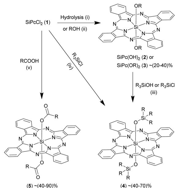
Scheme 4 Reactions of \text{SiPcCl}_2 , ( 1 ) where axial chlorides are replaced by alcohols, phenols, silanes and carboxylic acids. Reagents and conditions: (i) \text{NaOCH}_3 , 95% \text{CH}_3\text{CH}_2\text{OH} , reflux, 1 h; (ii) ROH, toluene, pyridine or sodium hydride, reflux, 120 °C, 24–96 h; (iii) \text{R}_3\text{SiOH} or \text{R}_3\text{SiCl} , toluene, pyridine, reflux, 120 °C, 3–6 h; (iv) \text{R}_3\text{SiCl} , NaOH, Aliquat HTA-1, chlorobenzene, reflux, 132 °C; (v) \text{RCOOH} , methoxyethyl ether, reflux, 160 °C, 0.5–6 h. R represent aryl or alkyl groups.
