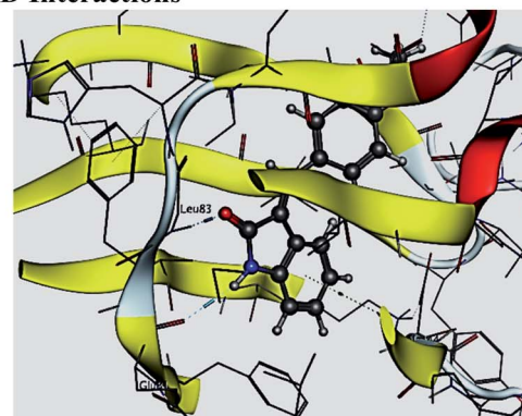
Fig. 8 2D and 3D ligand interactions of (A) co-crystallized sunitinib ( Z ) with CDK2, (B) 5a ( Z -diastereomer), (C) compound 6c ( E -diastereomer). All ligands are docked into the active site of CDK2 (PDB ID: 3T11).
