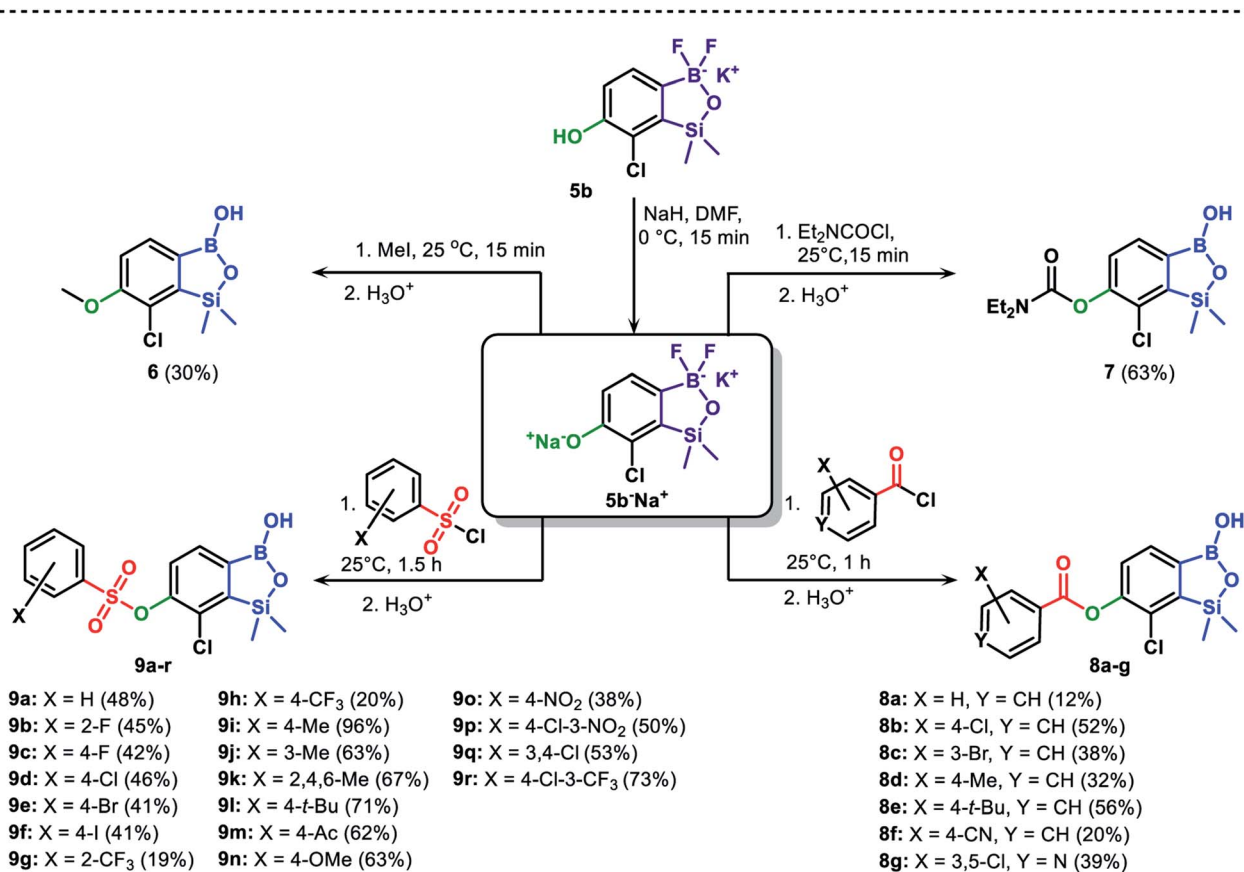
Scheme 2 Synthesis of functionalized benzosiloxaboroles 6 , 7 , 8a–8g , 9a–9r .
