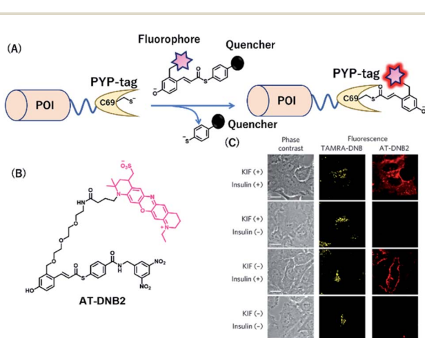
Fig. 6 (A) Schematic representation of a PYP-tag-based protein tag with chemical probe. (B) Structure of AT-DNB2, a NIR PYP-tag chemical probe. (C) Dual-color imaging of GLUT4 expressed in HeLa cells treated with kifunensine (KIF), which inhibits glycan maturation. Orange and red fluorescence signals in the images are derived from GLUT4 labeled with the TAMRA probe and AT-DNB2, respectively. POI, protein of interest. Reproduced from ref. 58 with permission from [Springer Nature], copyright [2016].
