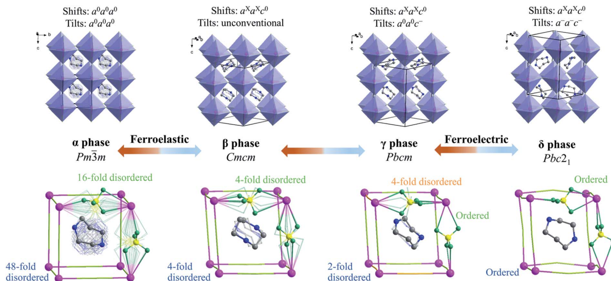
Fig. 2 Crystal structures of 1 at four phases. The blue and aqua (or orange) notes mark the different states for \text{H}_2\text{hpz}^{2+} organic cations and \text{BF}_4^- bridging ligands, respectively. The K, C, N, B, and F atoms are shaded in purple, gray, blue, yellow, and dark green, respectively. For clarity, H atoms are omitted, and only crystallographically independent \text{BF}_4^- anions are shown while the rest are simplified into aqua or orange bars.
