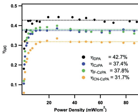
Fig. 5 Upconversion quantum efficiencies measured for 0.25 mM acceptors/annihilators sensitized by \text{Zr}(\text{Me}_5\text{PDP}^{\text{Ph}})_2 ( \text{OD}_{514\text{nm}} = 0.2 ) in deaerated THF solutions as a function of excitation power density at 514.5 nm.
