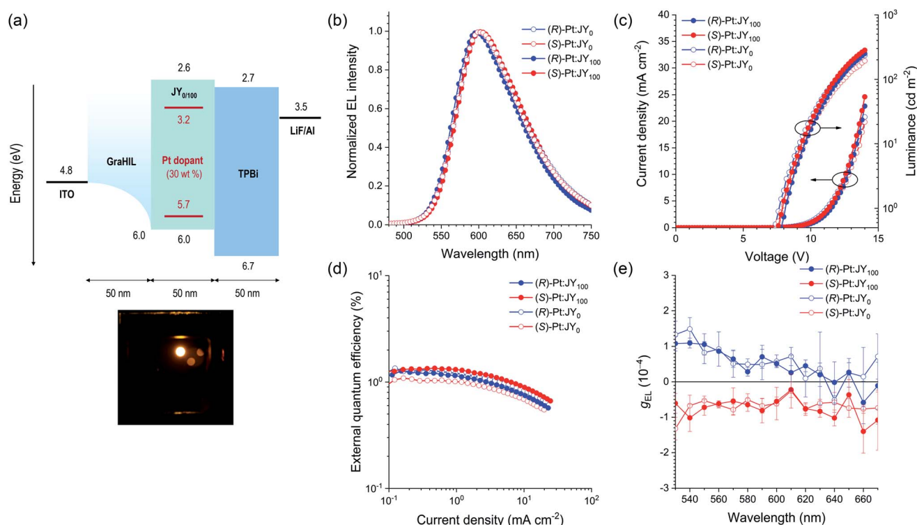
Fig. 9 (a) Energy-level diagram and device structure for the PLEDs with (R)- or (S)-Pt:JY n emitting layers. The positions of the energy levels of the polymer hosts were determined with cyclic and differential pulse voltammetry, and the positions of the other levels have previously been reported. 89–91 The bottom photo shows the electroluminescence of the device. (b) Electroluminescence spectra recorded at a current density of 1.6 mA cm -2 . (c) Current density–voltage–luminance and (d) external quantum efficiency–current density characteristics of the PLEDs. (e) Spectra of g EL recorded at a current density of 2.2 mA cm -2 averaged over 20 measurements. The error bars represent standard deviations.
