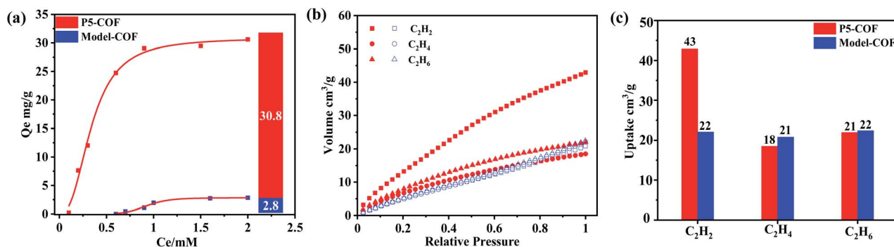
Fig. 2 (a) Langmuir adsorption isotherms of paraquat by P5-COF and Model-COF . Inset: the comparison of the paraquat adsorption capacity of P5-COF and Model-COF ; (b) gas adsorption isotherms of P5-COF (red) and Model-COF (blue) at 273 K; (c) comparison of gas adsorption uptakes of P5-COF and Model-COF at 273 K.
