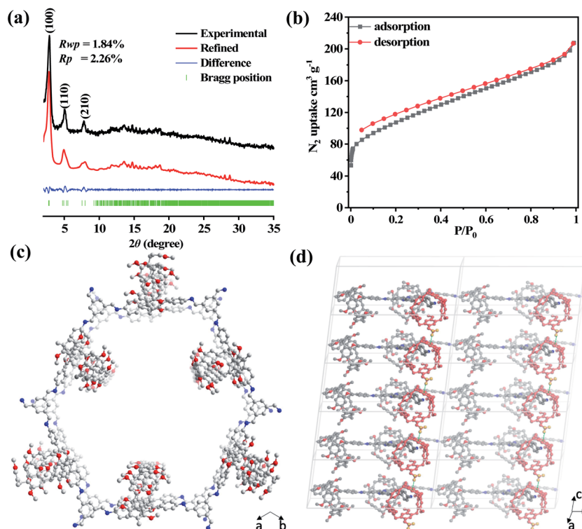
Fig. 1 (a) Experimental and simulated PXRD patterns of P5-COF ; (b) N_2 adsorption isotherms of P5-COF at 77 K; (c and d) top view (c) and side view (d) of P5-COF in the AA stacking model. The green dash indicates the CH- \pi stabilizing interactions.
