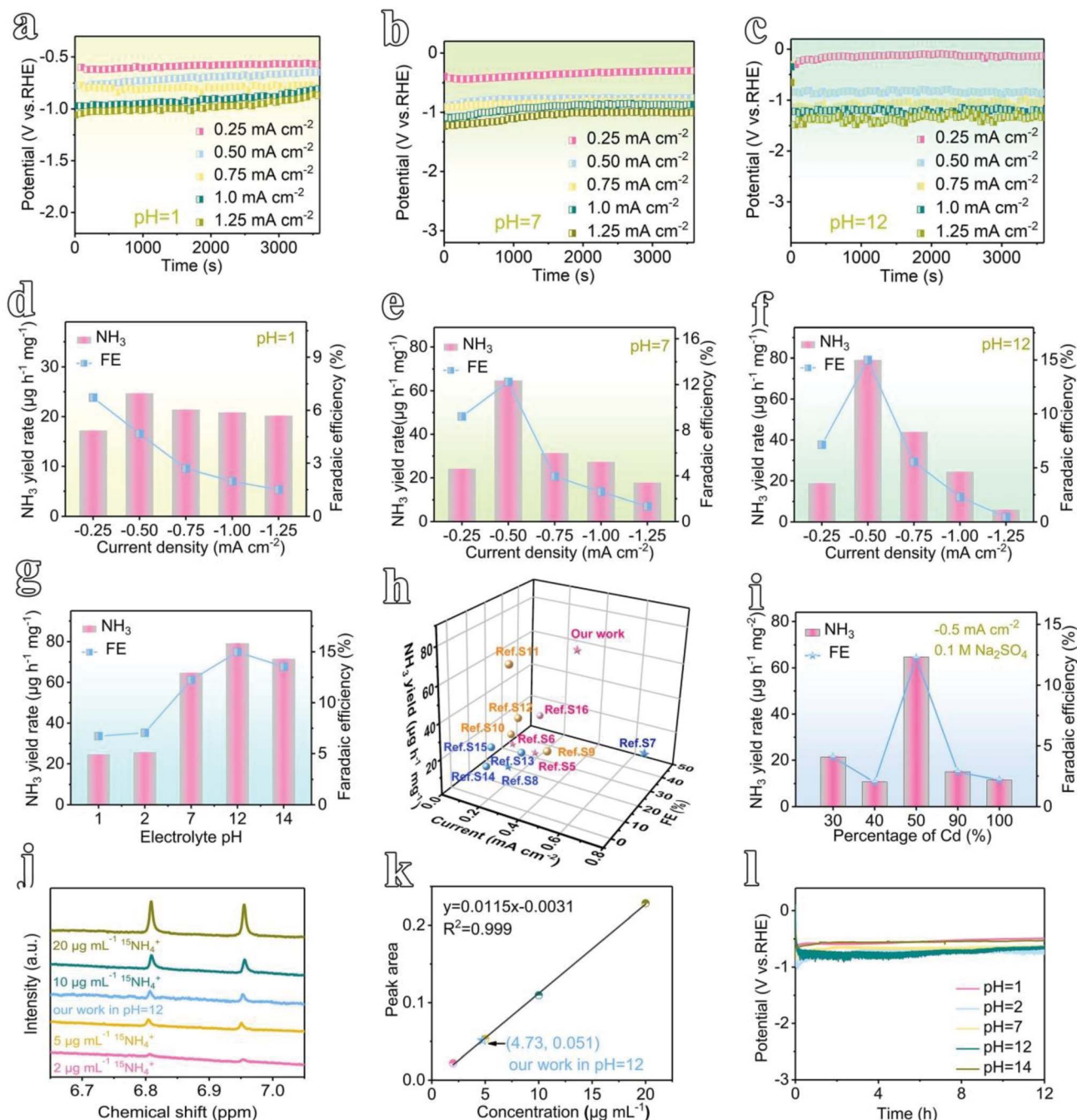
Fig. 3 The nitrogen electroreduction performance of 2D In-MOF at all pH values. The chronoamperometric curves at pH values of (a) 1, (b) 7, and (c) 12. (d–f) The corresponding NH 3 yield rates and faradic efficiencies (FEs) at different applied current densities. (g) NH 3 yield rates and FEs at different pH values (the applied current is -0.5 mA cm -2 ). (h) A comparison of the NRR activity of our sample with several state-of-the-art electrocatalysts. These electrocatalysts have been marked in different colours according to the different pH values of the electrolytes used, where alkaline is pink, neutral is blue, and acidic is yellow. (i) A comparison of the activities of In-MOF samples prepared using different amounts of Cd precursor in the synthetic process. (j) 500 MHz 1 H NMR spectra of NRR products tested using 15 N 2 feed gas and (k) the calibration curve of the 15 NH 4 + benchmark material. (l) Stability testing for 12 h at different pH values (the applied current is -0.5 mA cm -2 ).
