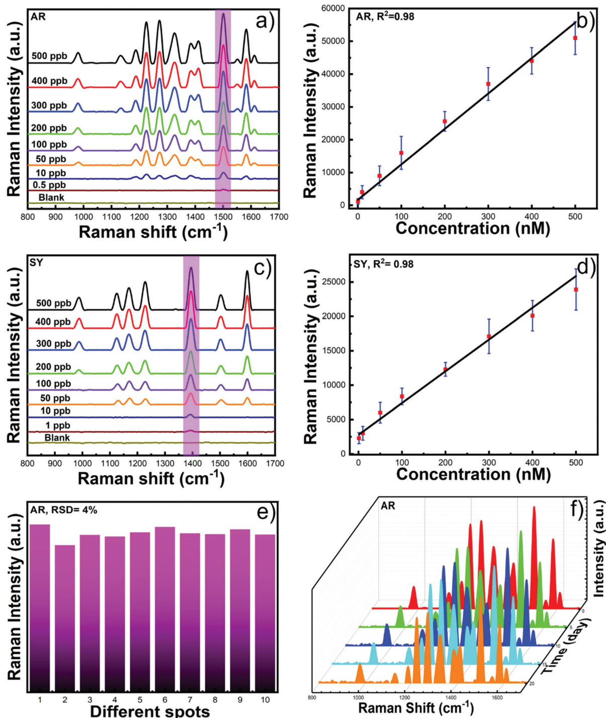
Fig. 3 SERS spectra of AR using GNS-5 at different concentrations from 500 ppb to 0.5 ppb (a). The calibration curve for the characteristic peak intensity at 1500 cm -1 as a function of AR concentration (b). SERS spectra of SY at different concentration from 500 ppb to 1 ppb (c) and SERS intensity of SY at 1395 cm -1 as a function of different concentrations (d). SERS reproducibility of allura red using GNS-5 (e). Representative SERS spectra of GNS-5 after 20 days measured with 5 days interval showing good stability of GNS-5 (f).
