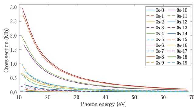
Fig. 8 Vibrational resolved cross sections for measurements in the ultracold regime ( 0s initial state) and ammonia's valence shell.
