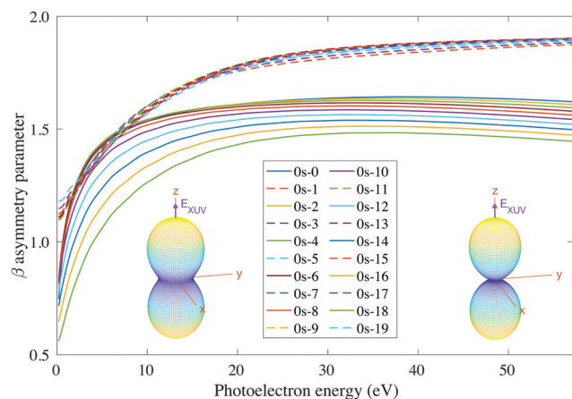
Fig. 9 Vibrational resolved \beta parameter for measurements in the ultracold regime ( 0s initial state) and ammonia's valence shell. Inset figures: corresponding photoelectron angular distributions for the \nu' = 16 vibrational state of the cation at a photoelectron energy of 2 eV (left) and 50 eV (right).
