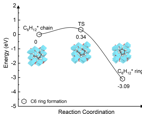
Fig. 8 Energy profile of the ring formation from the carbon chain \text{C}_6\text{H}_{12}^* species on the \gamma - \text{Al}_2\text{O}_3(100) surface.
