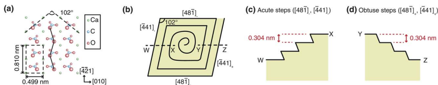
Fig. 1 Models of the calcite ( 10\bar{1}4 ) surface. (a) Atomic-scale surface structure consisting of \text{Ca}^{2+} and \text{CO}_3^{2-} . (b) Step arrangement around a screw dislocation during the calcite growth. (c) Acute steps. (d) Obtuse steps.
