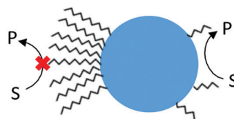
Fig. 8 (a) Scheme showing that proper energetic alignment allows a driving force for electron transfer. (b) Overlap between the quantum dot photoluminescence spectrum and the energy accepting ligand absorbance spectrum is required for energy transfer. (c) Physical separation between the nanocrystal core and the energy or charge accepting moiety can control the rate of forward, and by extension, backward transfer. (d) Long, dense ligand shells can prevent substrate access to the nanocrystal. Shorter, less dense ligands allow close interaction between the nanocrystal and substrate, promoting catalysis.
