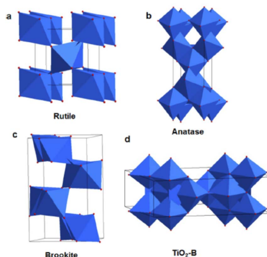
Fig. 4 Schematic unit cell structure of four TiO_2 polymorphs: (a) rutile (b) anatase (c) brookite and (d) TiO_2 -B 66 (Reprinted with permission from ref. Wang, X. et al. , 2014. Copyright 2014 American Chemical Society).
