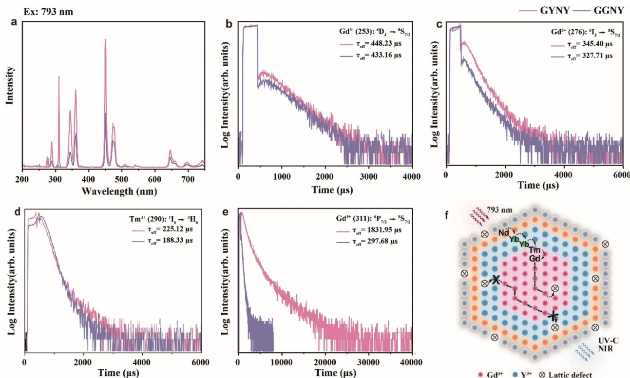
Fig. 3 (a) Upconversion emission spectra of GYNY and GGNY nanocrystals under 793 nm excitation. (b and c) Upconversion luminescence decay curves of \text{Gd}^{3+} emissions at 253 nm and 276 nm in GYNY and GGNY by pulsed 793 nm excitation. (d and e) Upconversion luminescence decay curves of \text{Tm}^{3+} emissions at 290 nm and \text{Gd}^{3+} emission at 311 nm in GYNY and GGNY by pulsed 793 nm excitation. (f) Schematic illustration of the energy transfer mechanism for UVC and NIR generation within the GYNY heterogeneous nanocrystal.
