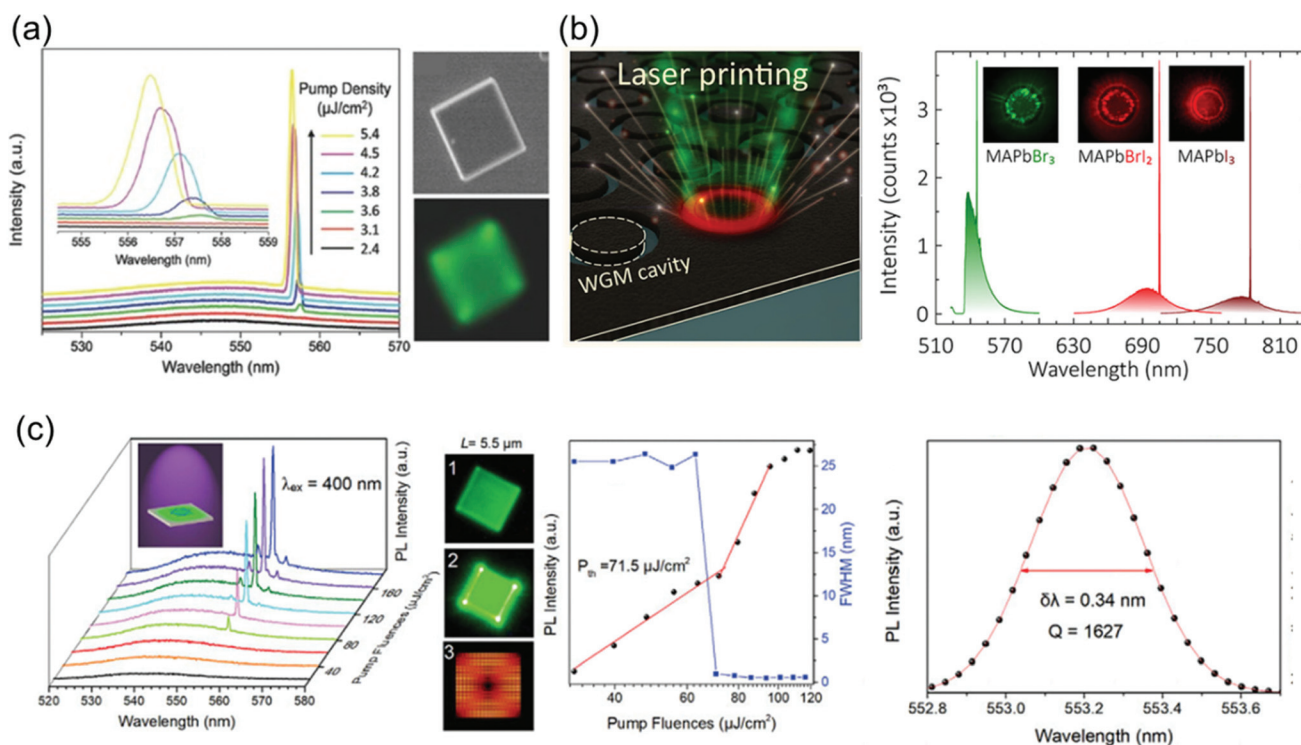
Fig. 18 (a) PL spectra of a square-shaped microdisk with a footprint of 2.0 × 2.0 × 0.6 μm 3 as shown in the optical and PL intensities measured as a function of excitation density at 400 nm. Inset is the enlarged PL spectra between 555 and 559 nm. Reproduced with permission. 46 Copyright 2015, Wiley-VCH. (b) Schematic of the large-scale arrays of perovskite microlasers and their photoexcitation. Optical images of the perovskite microlasers of different compositions and their lasing spectra: MAPbI 3 (brown curve), MAPbBrI 2 (red curve), and MAPbBr 3 (green curve). Reproduced with permission. 47 Copyright 2019, ACS. (c) Pump-fluence-dependent PL spectra of a single FAPbBr 3 square-shaped microdisk with edge length ( L ) of ≈ 5.5 μm under 400 nm (1 kHz, 100 fs) excitation. The inset shows schematic of an FAPbBr 3 square-shaped microdisk on a glass substrate, pumped by a 400 nm excitation wavelength. Fluorescence images of (1) below and (2) above the lasing threshold. (3) Simulated electric-field distribution, | H z |, inside the square-shaped perovskite cavity under a transverse electric resonant mode. Pump-fluence-dependent PL intensity and FWHM of a lasing oscillation mode at 553.2 nm. Reproduced with permission. 48 Copyright 2020, Wiley-VCH.
