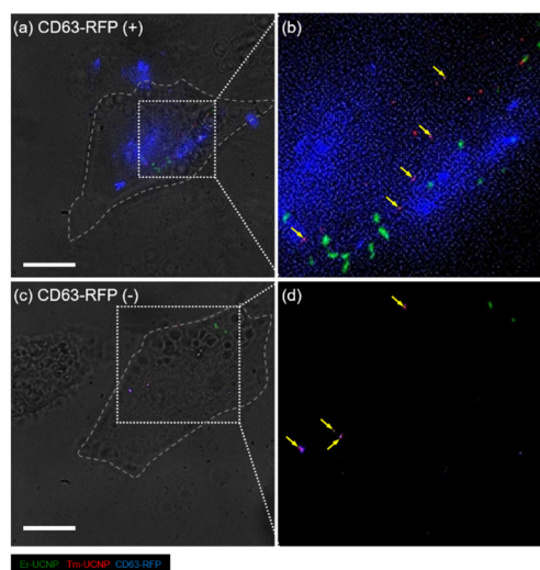
Fig. 4 Super-resolution radial fluctuation (SRRF) images of CD63-RFP-expressed and wild-type HeLa cells containing UCNPs. (a) Merged image of Er-UCNPs, Tm-UCNPs, and CD63-RFP in CD63-RFP expressed HeLa cells. White dotted line shows the cell boundary. (b) Magnified image of the white box in (a) without the bright-field image. (c) Merged image of Er-UCNPs, Tm-UCNPs, and CD63-RFP in wild-type HeLa cells. White dotted line shows the cell boundary. (d) Magnified image of the white-dashed box in (c) without the bright-field image. Yellow dots marked with the yellow arrows show the co-localization of Tm-UCNPs with CD63-RFP. Scale bars represent 10 \mu m.
