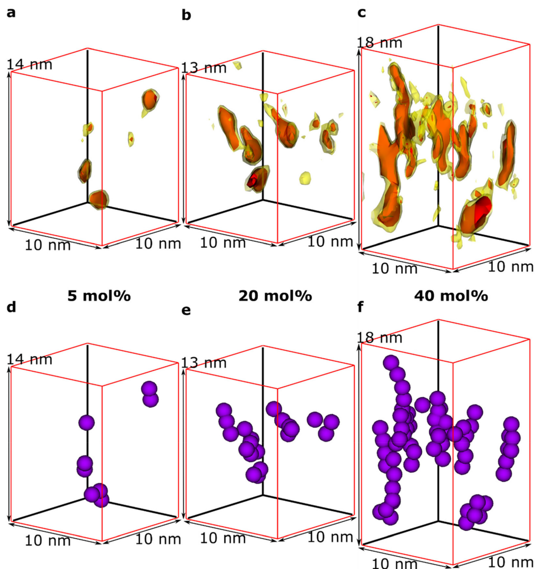
Fig. 3 Representative sub-volumes of the tomographic reconstructions of p(g42T-T) doped with 5, 20, and 40 mol% Mo(tfd-COCF 3 ) 3 , respectively. (a–c) Reconstructed sub-volumes showing the clusters and (d–f) markers indicate the positions of individual Mo(tfd-COCF 3 ) 3 species in the clusters and visualise the gradual change in cluster morphology.
