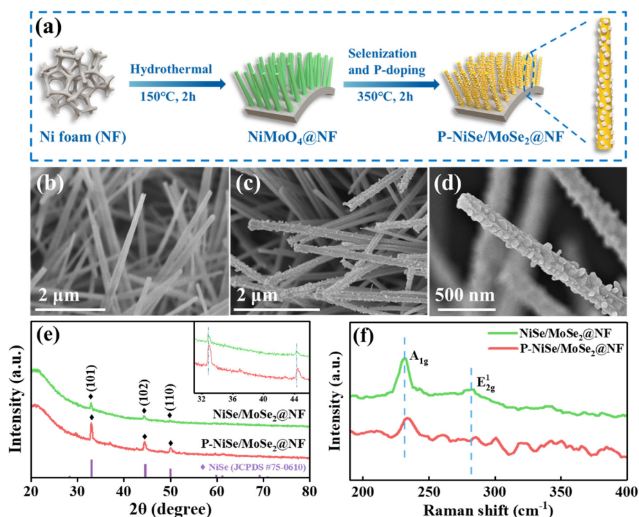
Fig. 1 (a) Schematic of the synthesis of the P-NiSe/MoSe 2 @NF electrode. SEM images of (b) NiMoO 4 @NF and (c) and (d) P-NiSe/MoSe 2 @NF. (e) XRD patterns and (f) Raman spectra of NiSe/MoSe 2 @NF and P-NiSe/MoSe 2 @NF.
