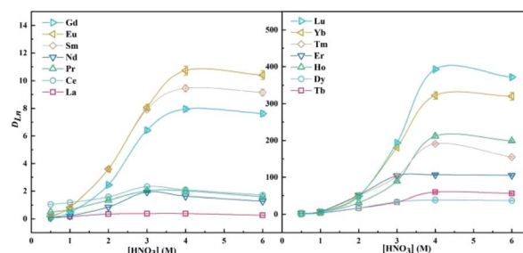
Fig. 3 Effect of HNO 3 on the extraction of Ln(III) by L II in 40/60 (v/v)% n -octanol/kerosene (O : A = 1 : 1, [Ln 3+ ] init = 3 mM).
