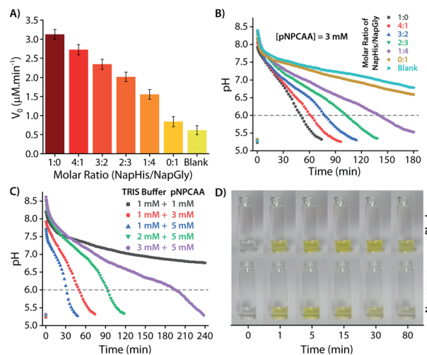
Fig. 6 (A) Rate of hydrolysis of pNPCA (0.5 mM) using different molar ratios of NapHis/NapGly ([nanozyme] = 100 \mu\text{M} ) in pH 8 buffer. (B) pH clock using different molar ratios of NapHis/NapGly nanozyme (100 \mu\text{M} ), 1 mM pH 9 TRIS buffer and 3 mM pNPCAA. (C) pH clock using various molar ratios of pH 9 TRIS buffer and pNPCAA in the presence of 100 \mu\text{M} nanozyme. (D) Photographic images of the nanozyme and blank (without nanozyme) solution captured along the course of the pH clock triggered by using 0.5 mM pH 9 TRIS buffer and 1 mM pNPCAA.
