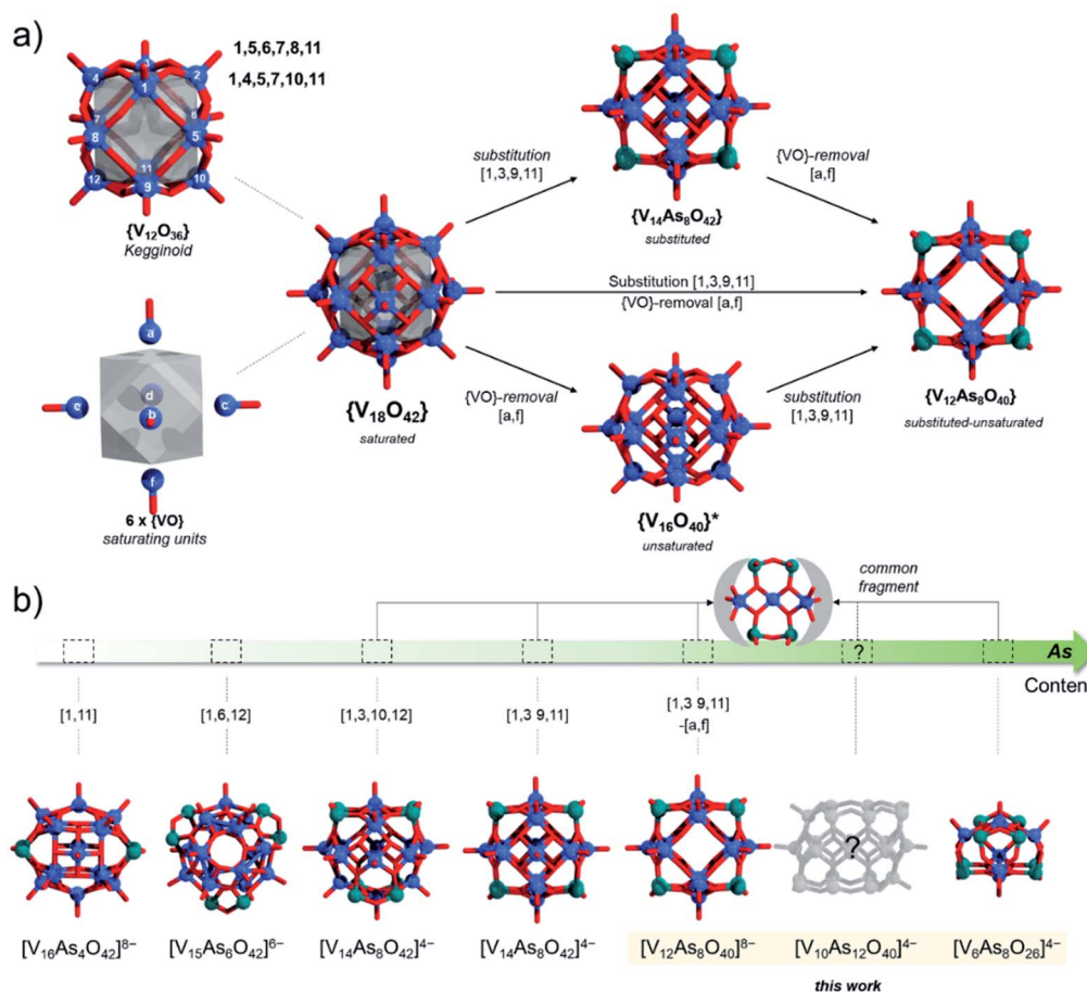
Fig. 2 Combination of ball-and-stick and schematic illustrations presenting (a) from left to right: the enumeration of the eighteen V centres in the kegginoide \alpha\text{-}\{V_{18}O_{42}\} , the kegginoide \alpha\text{-}\{V_{18}O_{42}\} archetype, its substituted, unsaturated and substituted-unsaturated derivatives. For \{V_{16}O_{40}\} , the experimentally known structure derives from \beta\text{-}\{V_{18}O_{42}\} ; (b) gradual ordering of the different As-POVs according to increasing arsenic content. The substitution and \{VO\} removal configurations from \{V_{18}O_{42}\} are provided in parentheses. Colour code: V = blue, O = red and As = green spheres.
