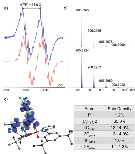
Fig. 7 (a) EPR spectra of [1\text{-OC}(\text{C}_6\text{F}_5)_2]^\bullet (blue) and its simulation (red); (b) MS of the reduced [1\text{-OC}(\text{C}_6\text{F}_5)_2]^\bullet (905.2927 (M) ^\bullet ) (red) and its simulation (blue); (c) DFT calculated Mulliken atomic spin densities in [1\text{-OC}(\text{C}_6\text{F}_5)_2]^\bullet .
