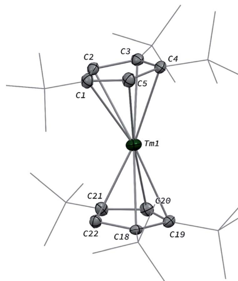
Fig. 2 Molecular structure of one of the two independent molecules of 1 in the solid state with thermal ellipsoids at the 40% probability level (except for the t\text{-Bu} groups depicted in wireframe). Only one disordered position for the t\text{-Bu} groups has been depicted and H atoms have been omitted for clarity. Selected bond distances (Å): Tm1–C1 2.712(4), Tm1–C2 2.676(4), Tm1–C3 2.681(4), Tm1–C4 2.664(4), Tm1–C5 2.670(4), Tm1–C18 2.673(4), Tm1–C19 2.677(4), Tm1–C20 2.686(4), Tm1–C21 2.703(4), Tm1–C22 2.658(4).
