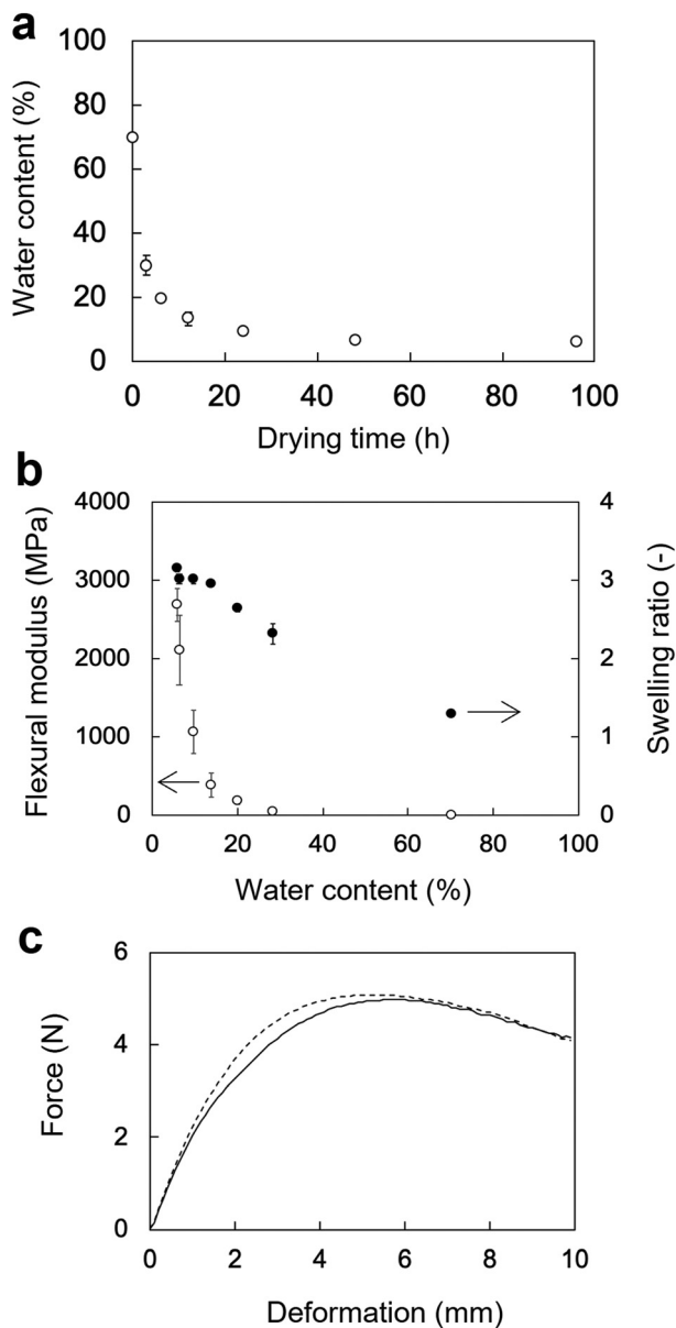
Fig. 4 (a) Water contents (WC) of rectangular PVA hydrogels as a function of drying time. (b) Flexural moduli and swelling ratios of rectangular PVA hydrogels as a function of WC. Data are presented as the mean \pm SD ( n = 3 ). (c) Force–deformation curves of the tube-shaped PVA hydrogel (solid line) and PS (dotted line).
