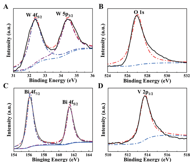
Fig. 3 XPS spectrum of the WO 3 /BiVO 4 heterojunction: (A) W 4f. (B) O 1s. (C) Bi 4f. (D) V 2p.
