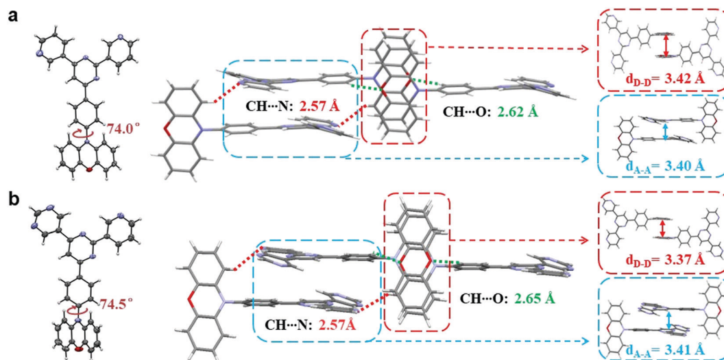
Fig. 3 Thermal ellipsoid drawing structures and intermolecular geometries of (a) PyPmP and (b) PmPmP in the single crystals determined by X-ray analysis. Abbreviations: d_{D-D'} and d_{A-A'} are the identity distances between the neighbor D and A moieties, respectively.
