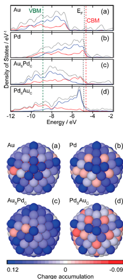
Fig. 22 (a–d) Electronic density of states (DOS) profiles of 147-atom icosahedral clusters of Au, Pd, Au 8 Pd C , and Pd 5 Au C , respectively. The total valence DOS (gray) is complemented by the contributions of the d-orbitals in both the core (red) and outer shell (blue) region. E_F of the metal clusters, conduction band minima (CBM), and valence band maxima (VBM) of TiO 2 are indicated by black and red dashed lines, respectively. 261 27B (a–d) Charge localization from the view of the (100) surface of 147-atom icosahedral clusters of Au, Pd, Au 8 Pd C , and Pd 5 Au C , respectively. The blue and red colors represent atoms with electron accumulation and depletion, respectively. Reprinted with permission from American Chemical Society. 177
