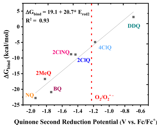
Fig. 3 Linear correlation between the DFT-calculated free energy of CO 2 binding and the experimental second reduction potential of the family of quinones in Fig. 1. The dashed line indicates the approximate potential of O 2 reduction in dry acetonitrile for comparison.
