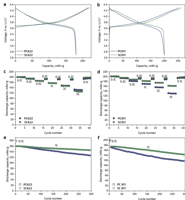
Fig. 3 Electrochemical characterization of the cathode materials: first-cycle voltage profile (a and b), rate capability tests (c and d) and cycling performance (e and f) of the single crystal SC622 and SC811 samples in comparison with their polycrystalline PC622 and PC811 analogues.
