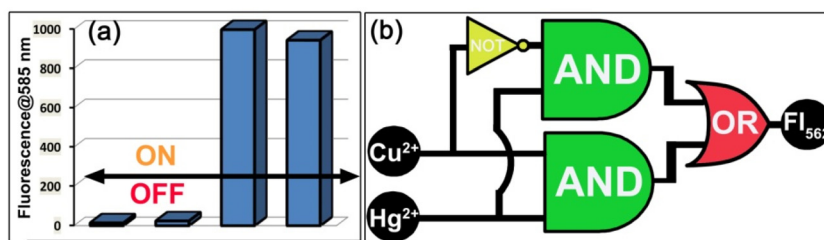
Fig. 11 (a) Optical bar responses and (b) corresponding schematic logic presentation of the TRANSFER logic gate based on the fluorescence responses of 1 at 562 nm, considering Cu 2+ and Hg 2+ as chemical inputs.
