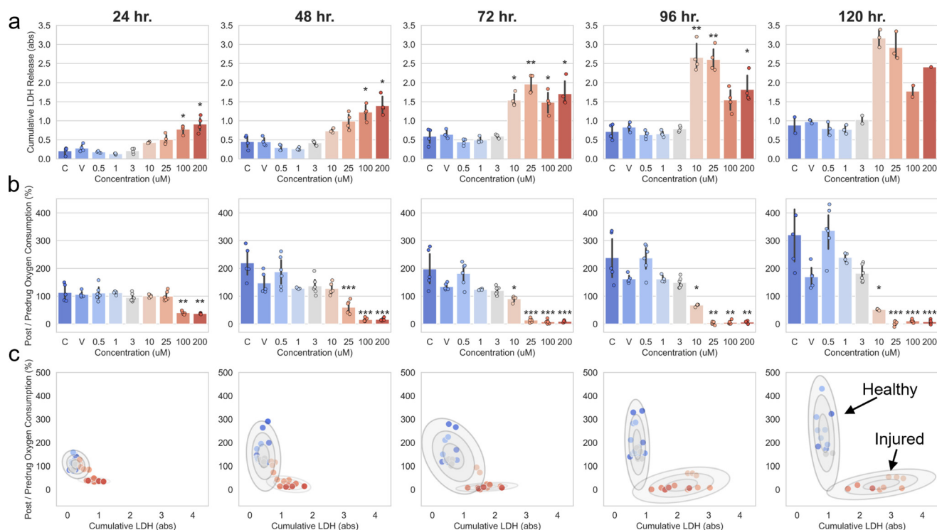
Fig. 5 Comparison between oxygen consumption and colorimetric-based cytotoxicity readouts for monitoring hRPTC injury in the mcPT. (a) Cumulative LDH in the hRPTC microchannel and (b) post/pre-drug oxygen consumption for each timepoint during exposure of hRPTCs to cisplatin for 5 days ( *p < 0.05 , **p < 0.01 , ***p < 0.0001 relative to untreated within each timepoint between 24–96 h using Kruskal–Wallis and Dunn's post-hoc test). There were insufficient replicates in cumulative LDH data at 120 h for statistical testing. (c) Unsupervised clustering of individual mcPTs into separate groups, representing healthy and injured tissue, at each timepoint based on post/pre-drug oxygen consumption and cumulative LDH data.
