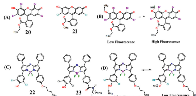
Fig. 14 (A) Molecular structure of fluorescent indicator dyes 20 and 21 and (B) their proposed fluorescence sensing mechanism of detection of NH 3 through acid–base equilibrium. (C) Molecular structure of aza-BODIPY sensors 22 and 23 and (D) their proposed fluorescence sensing mechanism of detection of NH 3 through acid–base equilibrium.
