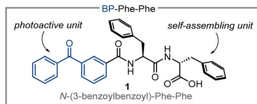
Scheme 1 Self-assembling photocatalyst with benzophenone (BP) and Phe-Phe.
