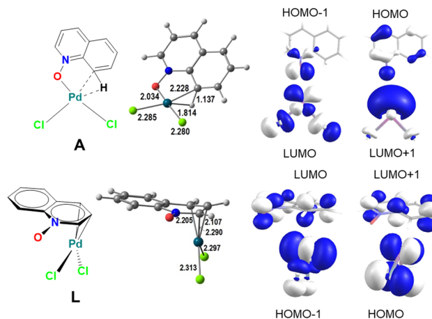
Scheme 4 The geometries of intermediates A and L (distances in Å) and the frontier molecular orbitals of QO and \text{PdCl}_2 relevant for their bond: A (top) and L (bottom).
