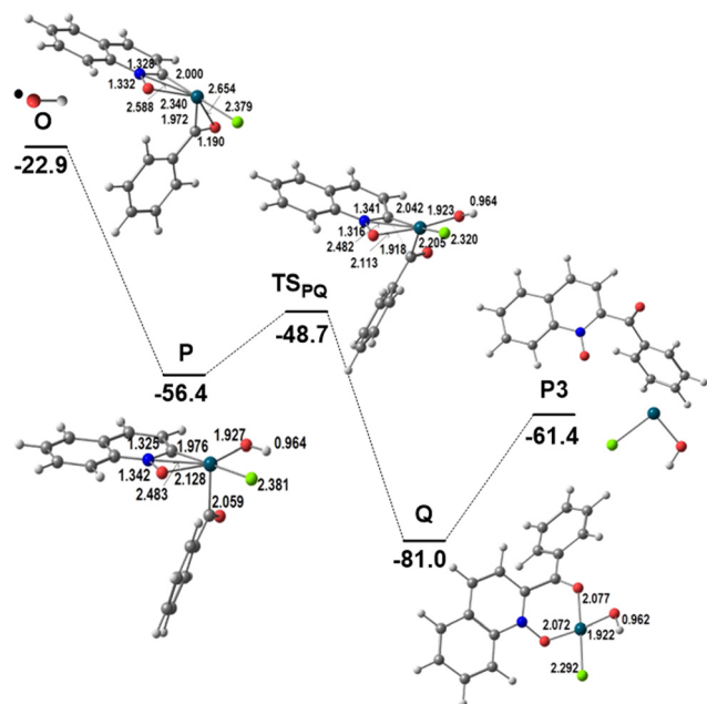
Fig. 6 Energy profile for the second part of the functionalization of QO at C2 (relative Gibbs energies in \text{kcal mol}^{-1} in dichloroethane; distances in Å).
