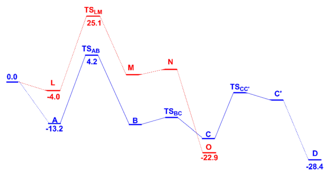
Scheme 3 The two energy profiles for the first steps in the C8 (blue) and C2 (red) activation reactions in dichloroethane with relevant Gibbs energies ( \text{kcal mol}^{-1} ).
