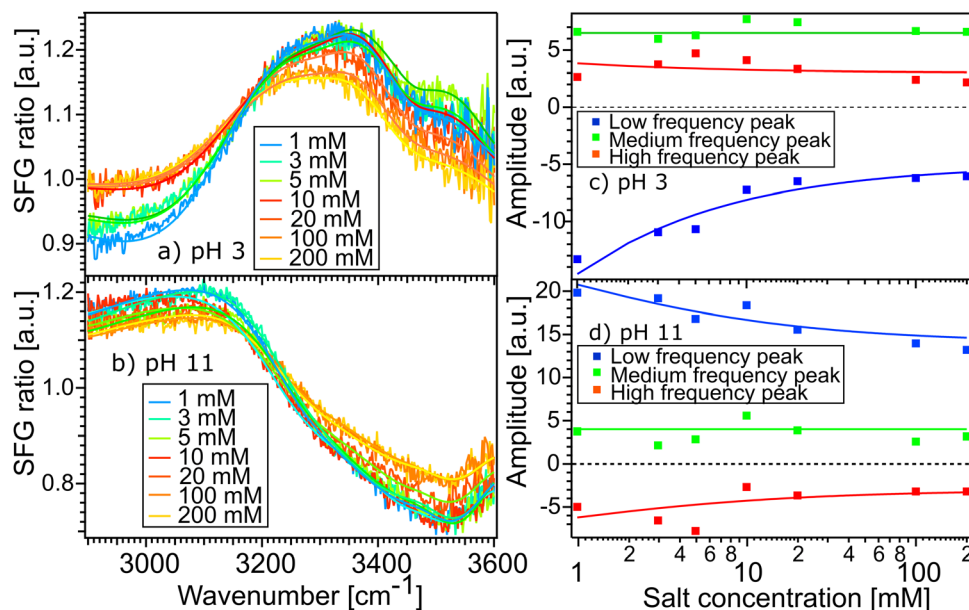
Fig. 5 SFG spectra of \text{H}_2\text{O} solutions of pH 3 (a) and pH 11 (b), with different NaCl concentrations, in contact with the STO layer. Amplitude of each peak obtained from fitting the SFG-spectra of water at pH 3 (c) and pH 11 (d), versus the ionic strength. The solid lines depict the data modelling based on the Gouy–Chapman model.
