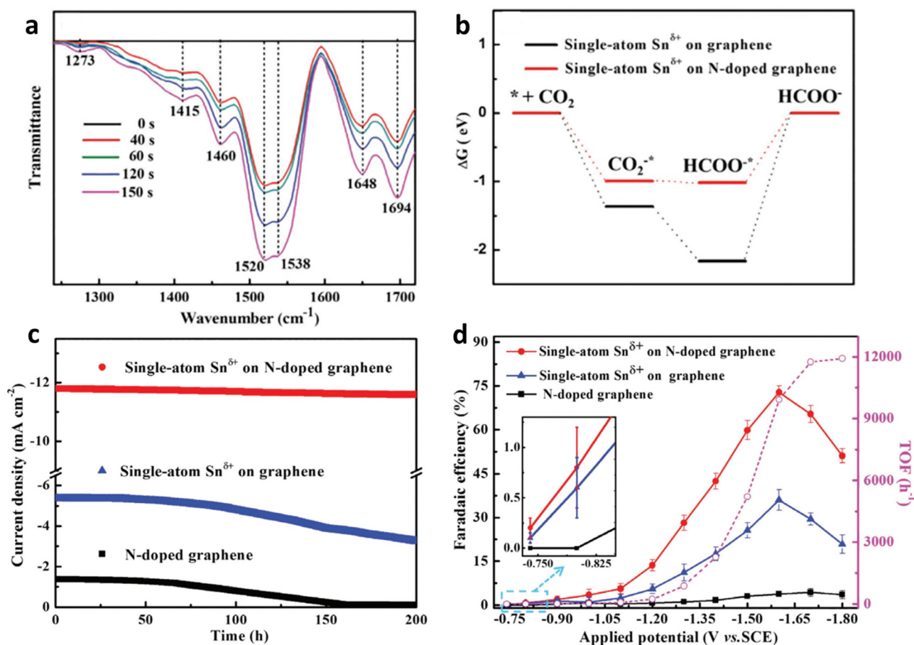
Fig. 5 (a) In situ FT-IR spectra of Sn-SACs. (b) Free energy diagrams. (c) Chronoamperometry tests at -1.6 V vs. SCE. (d) \text{FE}_{\text{HCOOH}} and TOF of the Sn-SACs. Reproduced with permission. 57 Copyright (2019) Wiley-VCH.
