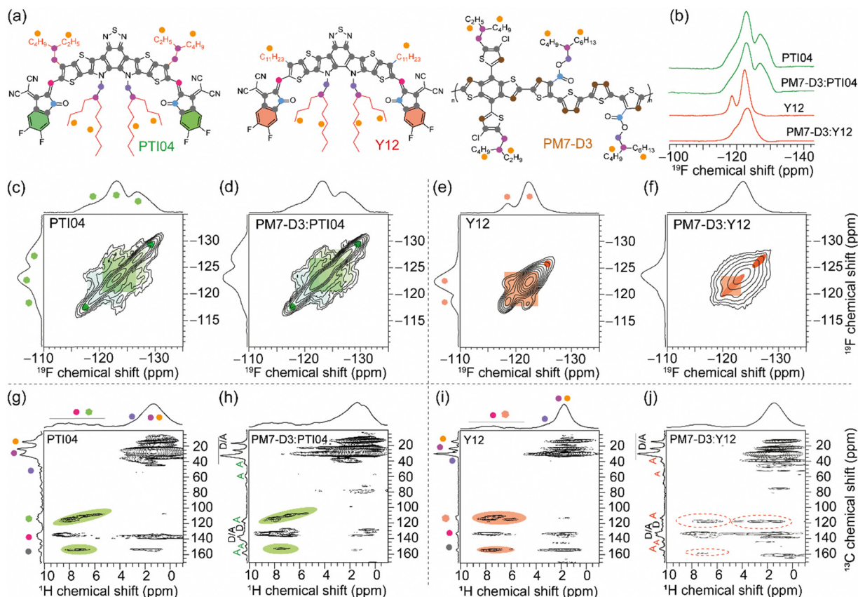
Fig. 5 (a) Structures of PM7-D3 , PTI04 , and Y12 with color dots to guide the analysis of 2D NMR spectra. (b) Solid-state 1D ^{19}\text{F} MAS NMR spectra of MA and PM7-D3:MA blends. Solid-state 2D ^{19}\text{F} – ^{19}\text{F} spin-diffusion NMR spectra of (c) neat PTI04 and (d) PM7-D3:PTI04 indicating the identical acceptor morphology, and (e) neat Y12 and (f) PM7-D3:Y12 blend films with different peak patterns highlighted in red. Solid-state 2D ^1\text{H} – ^{13}\text{C} HETCOR NMR spectra of (g) neat PTI04 and (h) PM7-D3:PTI04 indicating the identical local acceptor morphology as depicted by green ovals, and (i) neat Y12 and (j) PM7-D3:Y12 BHJ blend films showing the difference in the local morphology as depicted in the red dashed ovals.
