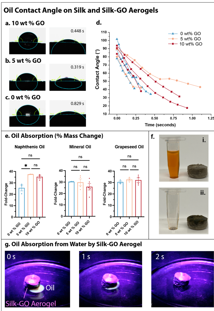
Fig. 4 Interactions of silk-GO aerogels with oil. (a–c) Representative contact angle of grapeseed oil on silk aerogels (10, 5, 0 wt% GO). (d) Average contact angle of grapeseed oil after contacting aerogel surface. (e) Oil adsorbed as fold change in mass for naphthenic oil, grapeseed oil and mineral oil for all conditions. Bar plot shows \bar{x} as mean values and error bars as standard error of the mean (SEM) ( N = 4 samples). Two-way ANOVA test, * denotes p < 0.05 . (f) Representative before and after images of total oil adsorption by silk aerogel with 10 wt% GO. (g) Representative images of oil adsorption from a container of water by a silk aerogel with 10 wt% GO over 2 s. For ease of visualization, oil has been labeled with a phosphorescent dye and illuminated with UV light.
