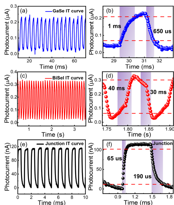
Fig. 4 The photoreponse to on/off irradiation showing (a, c, and e) the corresponding photodetector stability of GaSe, BiSel and the BiSel/GaSe heterojunction at V_{ds} = 2 V. (b, d, and f) The typical response speed of GaSe, BiSel and BiSel/GaSe heterojunction devices.
