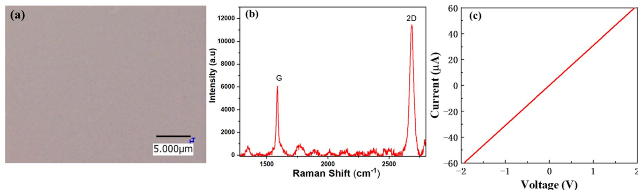
Fig. 3 (a) Optical image of transferred CVD graphene on the \text{SiO}_2/\text{black-36}^\circ\text{YX LiTaO}_3 substrate. (b) Raman spectrum of the CVD G-SAW sensor. (c) I - V characteristics of the fabricated G-SAW sensor.
