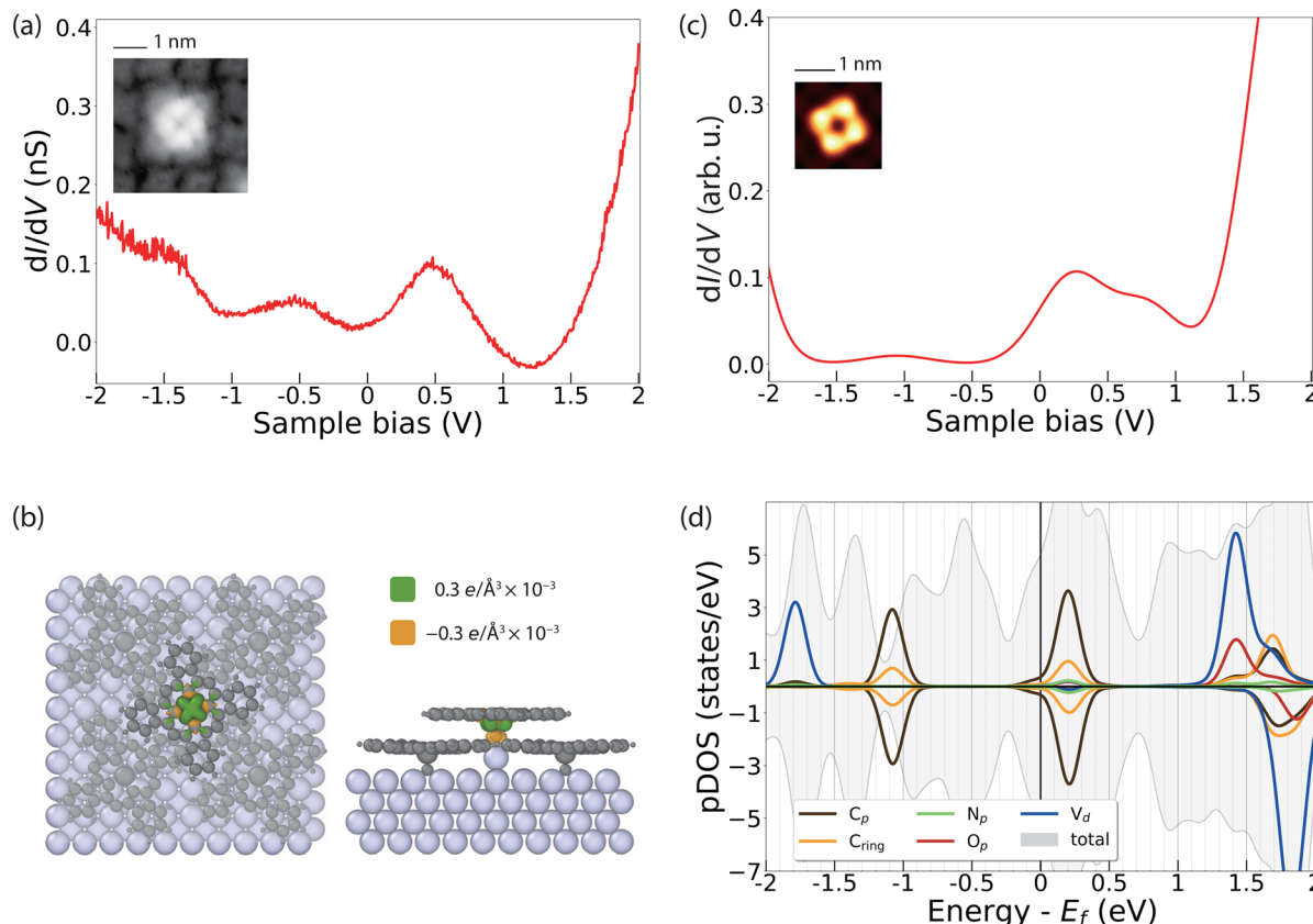
Fig. 4 Orbital structure of a single VOPc B molecule. (a) dI/dV curve measured at the centre of VOPc B ( V_{DC} = 1 V, I_{set} = 50 pA). (b) Top view (left) and side view (right) of DFT calculation of spin density of VOPc B molecule. The distribution of positive (green) and negative (orange) spin polarization is overlapped with the molecular structure. (c) Simulated dI/dV curve of VOPc B molecules with one silver atom added. (d) pDOS plot of VOPc B molecules projected on the orthogonalized atomic basis set. Inset in (a): STM topography of VOPc B (scan size of 3.9 \times 3.9 nm 2 , V_{DC} = 100 mV, I_{set} = 100 pA). Inset in (c): simulated topography of VOPc B (Image size of 1.44 \times 1.44 nm 2 , V_{DC} = 300 mV)
