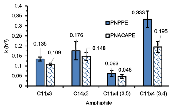
Fig. 5 Rate constants of PNPPE (blue, solid fill) and PNACAPE (blue, shingle pattern) depropargylation in presence of C11×3, C14×3, C11×4 (3,5) and C11×4 (3,4) metallic micelles.
