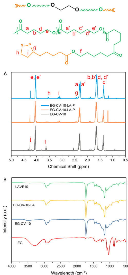
Fig. 1 (A) ^1\text{H} -NMR spectra of EG-CV-10, EG-CV-10-LA-F (full substituted), and EG-CV-10-LA-P (partly substituted); (B) FTIR of EG, EG-CV-X-LA, and LAVE.
