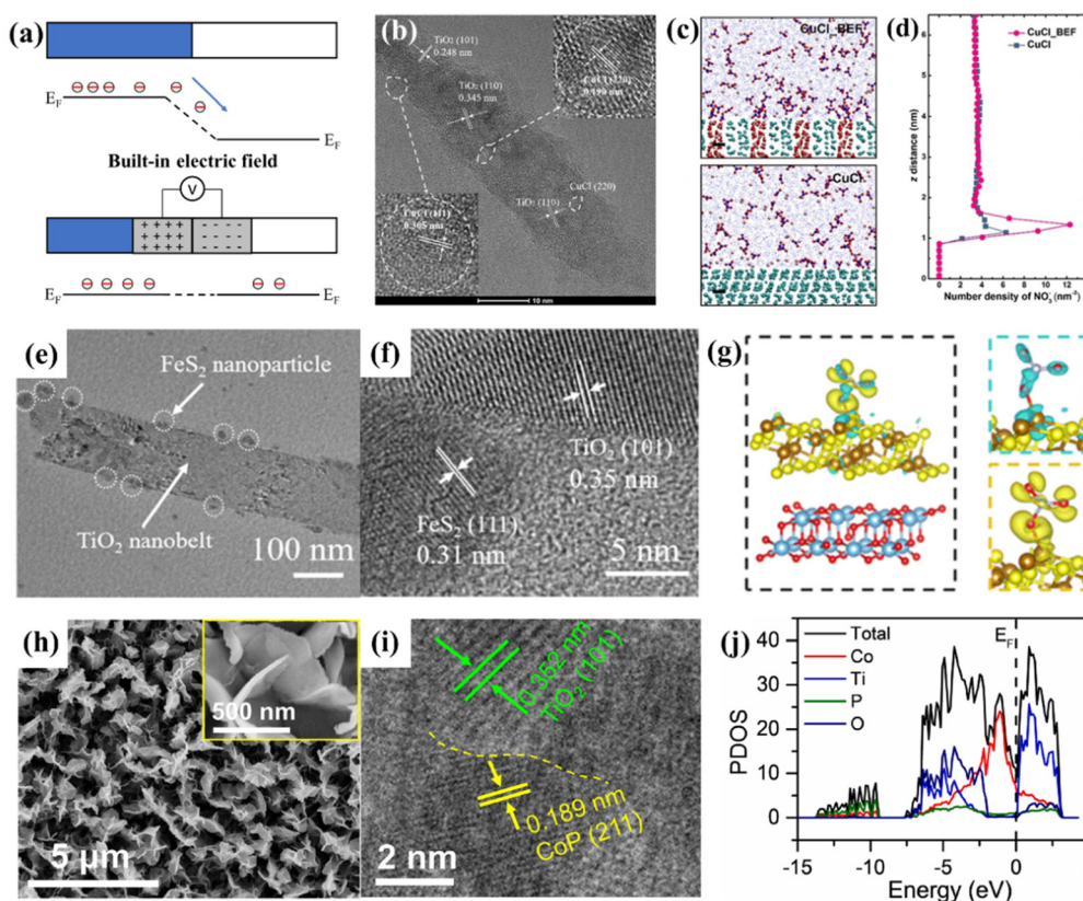
Fig. 5 (a) The formation of a built-in electric field at the heterostructure composed of two components with different Fermi levels. (b) Representative HRTEM image of \text{CuCl}_\text{BEF} . (c) Molecular dynamics simulation of \text{CuCl} and \text{CuCl}_\text{BEF} in \text{KNO}_3 ( 100 \text{ mg L}^{-1} ) solution. Scale bar, 0.5 \text{ nm} . (d) Distribution of \text{NO}_3^- along the z-axis electrode distance based on the molecular dynamics simulation. 72 Reproduced from ref. 72 with permission from Wiley-VCH, copyright 2022. (e) TEM and (f) HRTEM images of \text{FeS}_2 @ \text{TiO}_2/\text{TP} . (g) Charge density difference of \text{FeS}_2 @ \text{TiO}_2 with adsorbed \text{NO}_3^- , where yellow and cyan color indicate electron accumulation and depletion, respectively, and the isosurface values are set to 0.000213 \text{ \AA}^{-3} . 73 Reproduced from ref. 73 with permission from The Royal Society of Chemistry, copyright 2022. (h) SEM images and (i) HRTEM images of \text{CoP}/\text{TiO}_2 . (j) Calculated PDOS of \text{CoP}/\text{TiO}_2 . 76 Reproduced from ref. 76 with permission from Elsevier, copyright 2022.
