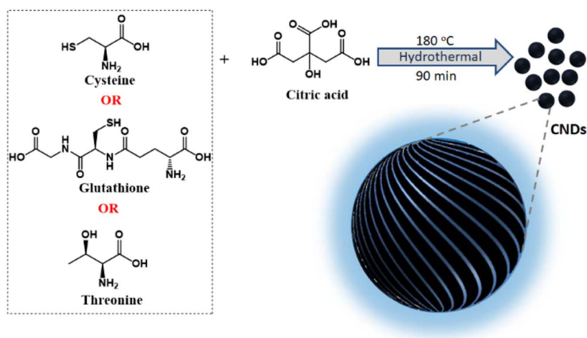
Fig. 1 Scheme illustrating the synthesis of chiral CNDs using a combination of citric acid and different chiral agents as precursors.
