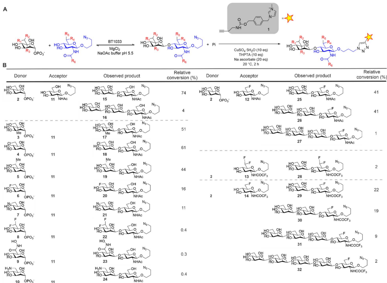
Fig. 2 (A) ITag screening methodology for BT1033 reactions. Reaction mechanism depicted in reverse phosphorylysis direction. (B) BT1033 activity towards unnatural donors and acceptors. 3,15
